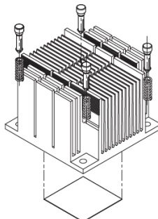
SPRING LOADED
